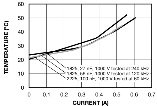
TEMPERATURE VS. RIPPLE CURRENT
