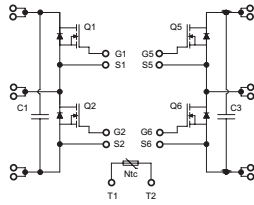
Full-Bridge Inverter
