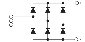
Three Phase Diode Bridge
