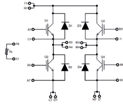
Full Bridge With Thermistor (VS-...MT...TFT)
