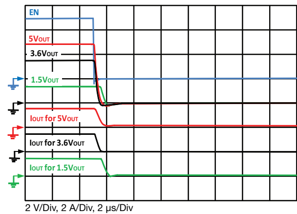
Fig. 20 - Typical Fall Time C OUT = 0.1 μF, C IN = 4.7 μF, I OUT = 1.5 A
