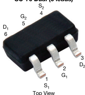
SOT-363 SC-70 Dual (6 leads)
