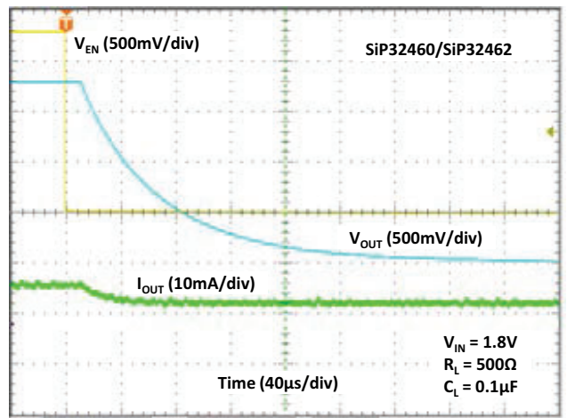
Fig. 36 - Turn-off Time
