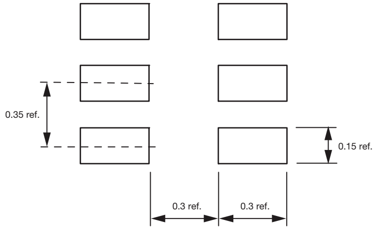
Mounting Footprint Dimensions in mm
