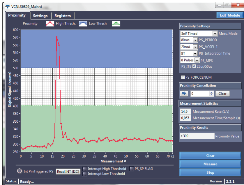
Fig. 30 - Upper and Lower Threshold Set and Hand in About 5 cm Distance
