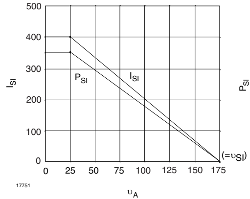
Fig. 3 - Dependency of Reliability Maximum Ratings on Ambient Temperature for SFH601, CNY174
