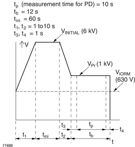
Fig. 1 - Measurement Method A of DIN EN 60747-5-5 (VDE 0884)
