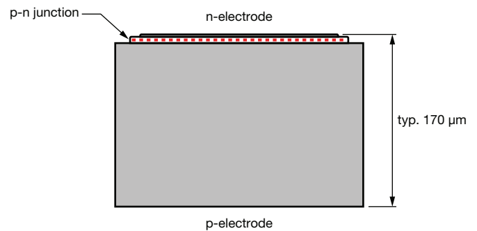
Fig. 3 - Sectional View
