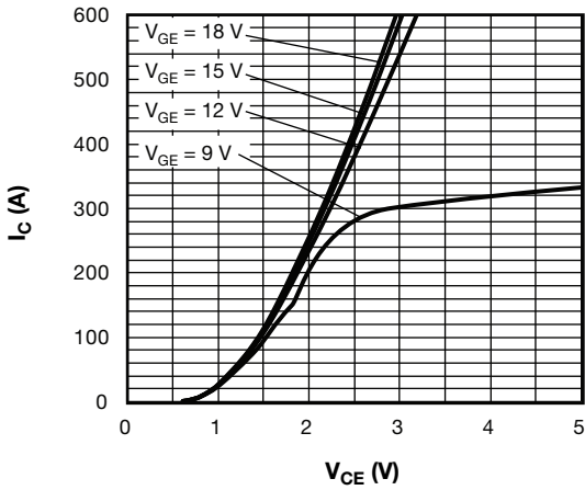
Fig. 2 - Typical IGBT Output Characteristics, T_J = 25\text{ }^\circ\text{C}
