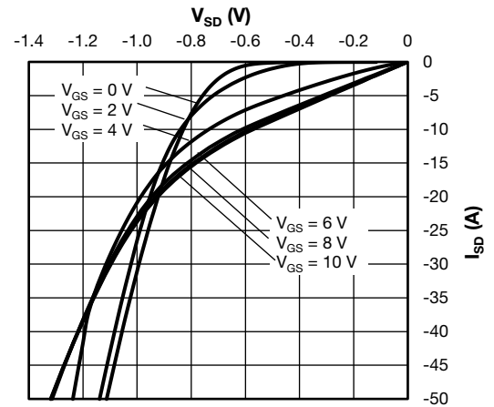
Fig. 10 - Typical MOSFET Source-to-Drain Current Characteristics at T_J = 25\text{ °C}
