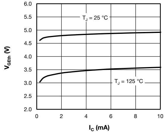
Fig. 5 - Typical Trench IGBT Gate Threshold Voltage
